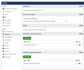
Fig. 4: Restrict the surfing area
