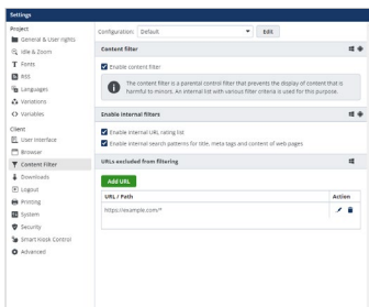
Fig. 5: Real time Internet content filter
