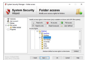
Fig. 2: Access rights for folders & files
